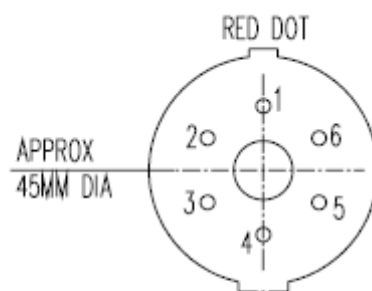
SHIP CONNECTOR – FIBRE ALLOCATION
